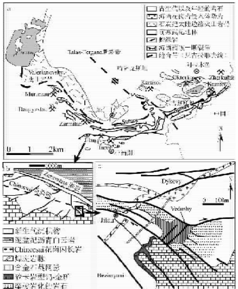
图4 中-南天山成矿省的构造线走向及其主要矿床分布(a), Zeravshan地区的Chinorsai背斜、Chinorsai花岗岩(b)和Jilau矿区地质简图(c) [69] Fig. 4 Strike of the lineament of the Centrao-South Tianshan metallogenic province and distribution of its related ore deposits (a), the Chinorsai anticline and Chinorsai granite in the Zeravshan area (b) and the geological sketch map of the Jilau deposit (c)
