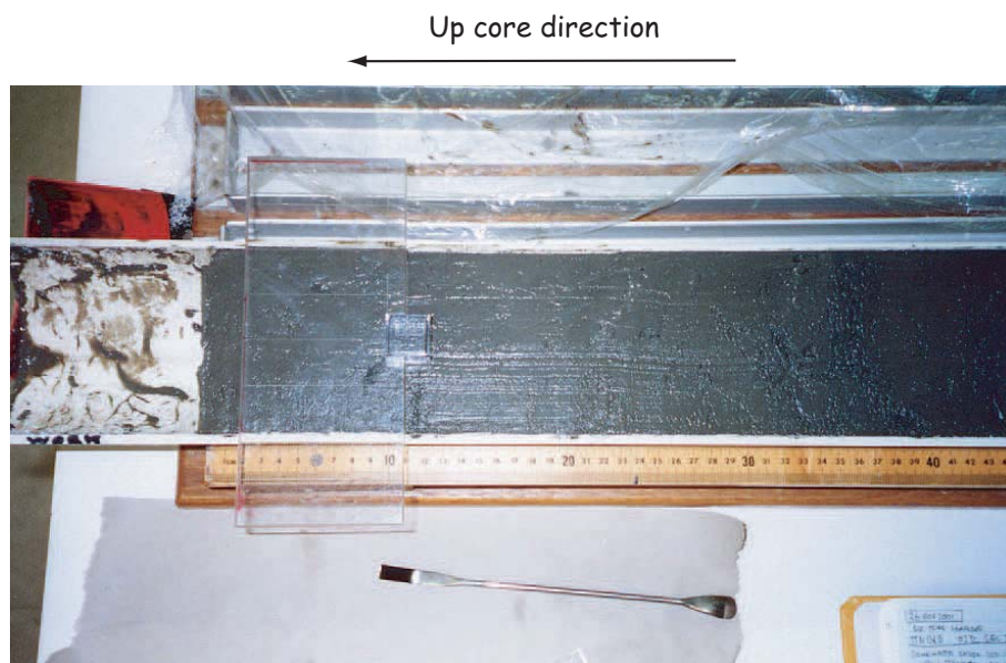
Figure 9.4: Sampling of a sediment core. A plastic cube with a hole in it to let the air escape is pressed into the split surface of a core. The orientation arrow points “up core”. After extraction, a label with the sample name is put on. Figure from Kurt Schwehr’s web site.
