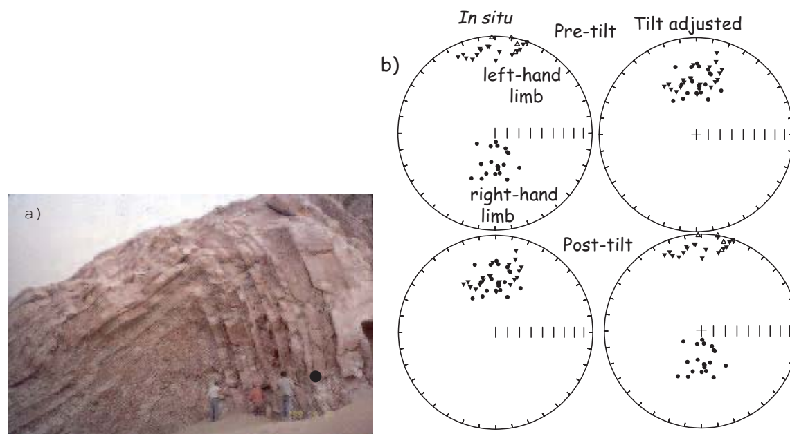
Figure 9.13: Sampling units with different bedding attitudes in the “fold test”. a) Example of folded beds. (Picture from Dupont-Nivet et al., 2002.) b) Hypothetical paleomagnetic directions are shown on equal area projections before and after adjusting for bedding tilt. Top pair represents the case in which the grouping of paleomagnetic directions is improved after adjusting for tilt which would argue for a pre-tilt acquisition of remanence. Lower pair represents a post-tilt acquisition of remanence in which the grouping is worse after restoring beds to the horizontal position.
