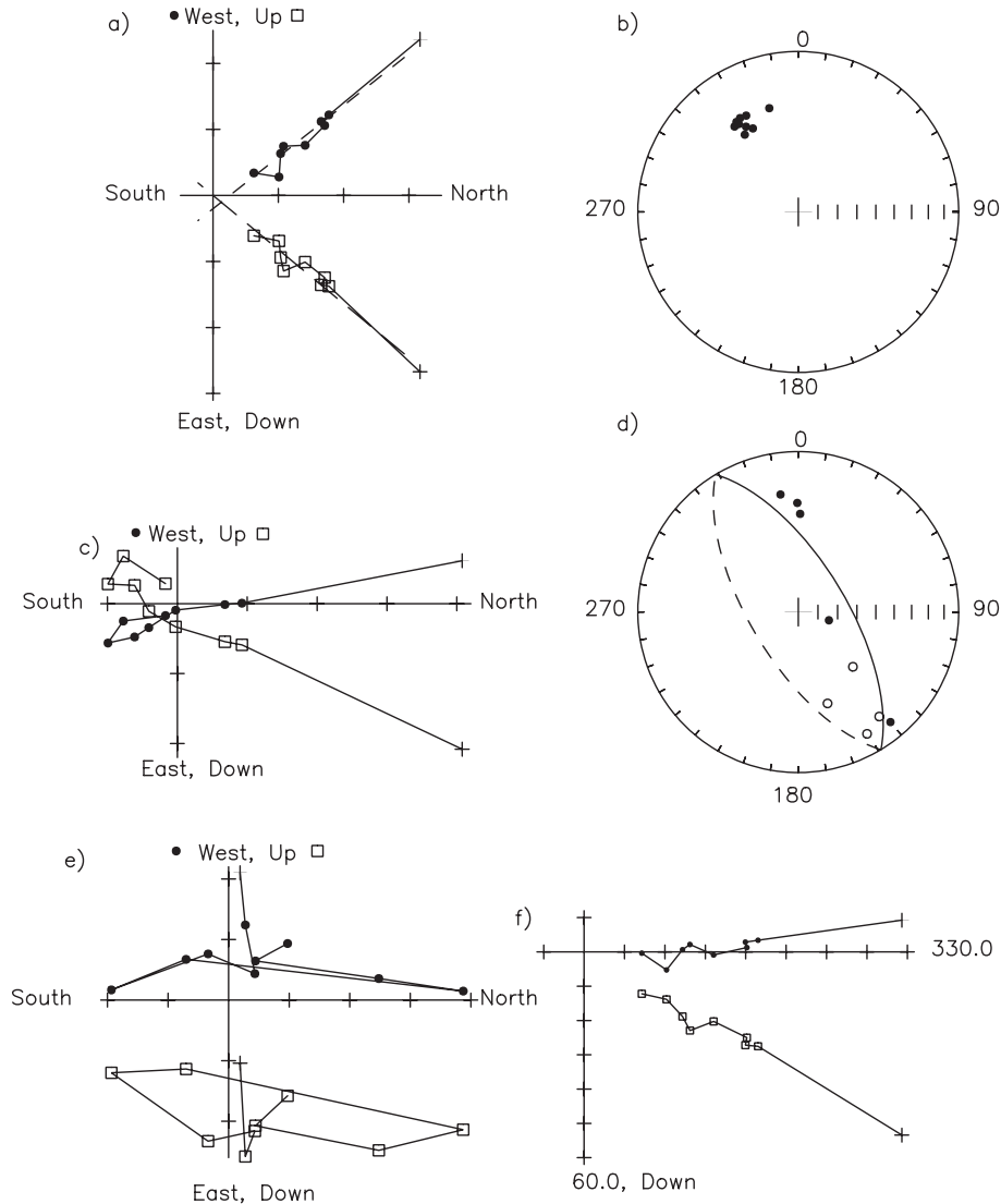
Figure 9.11: a) Orthogonal projection of data plotted with North on the horizontal axis. A single component of magnetization is present (see text). The horizontal projection is plotted with solid symbols and the vertical (North-down) component is plotted with open squares. The best-fit line through the data, as calculated by principal component analysis, is shown as a dashed line. b) Same data as in a), but plotted on an equal area projection. Solid (open) symbols are projections onto the lower (upper) hemisphere. c) Sample with two components that have overlapping stabilities. d) Same data as in c), but in an equal area projection. The trace of the best-fitting plane is shown, with a solid (dashed) line being a projection onto the lower (upper) hemisphere. e) Example of a complicated multi-component sample. f) Data from a) replotted with the horizontal axis along 330° instead of with respect to North.
