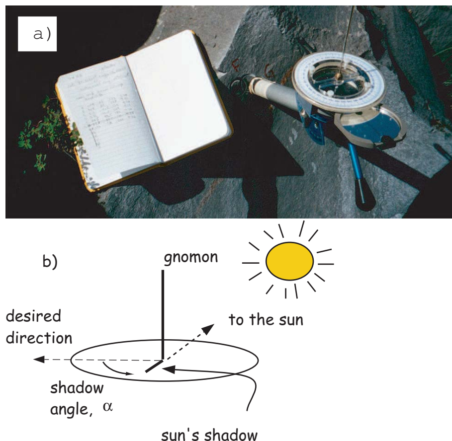
Figure 9.5: a) Pomeroy orientation device in use as a sun compass. b) Schematic of the principles of sun compass orientation.
