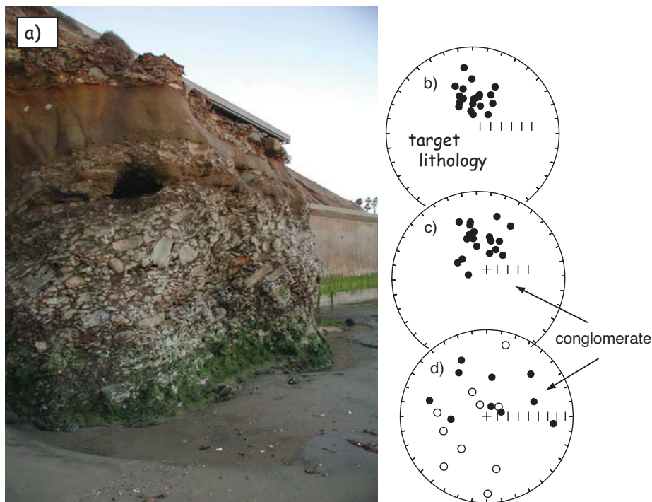
Figure 9.14: The paleomagnetic conglomerate test. a) The target lithology was involved in a catastrophic event leading to incorporation into a conglomerate bed. Samples are taken from individual clasts. The directions of samples from the target lithology are shown in b) indicating that it is relatively homogeneously magnetized. c) directions from the conglomerate clasts are also homogeneously magnetized; the magnetization must post-date formation of the conglomerate. In a positive conglomerate test d), the magnetization vectors of samples from the conglomerate clasts are random.
