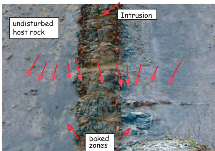
Figure 9.15: The baked contact test. In a positive test, zones baked by the intrusion are remagnetized and have directions that grade from that of the intrusion to that of the host rock. If all the material is homogeneously magnetized, then the age of the intrusion places an upper bound on the age of magnetization.
