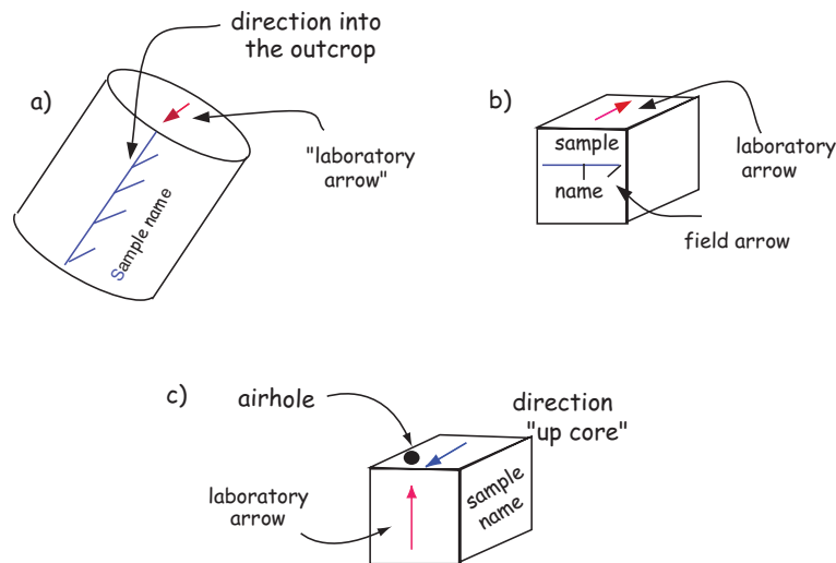
Figure 9.7: Various types of possible sample shapes and orientation conventions. a) A one inch slice from a drilled core. b) A cube of sediment sanded from a hand sample. c) A sample from a piston core.
