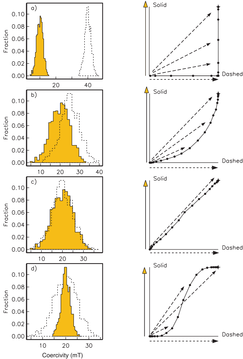
Figure 9.10: Principle of progressive demagnetization. Specimens with two components of magnetization (shown by heavy arrows on the right hand side), with discrete coercivities (plotted as histograms to the left). The original “NRM” is the sum of the two magnetic components and is shown as the + in the diagrams to the right. Successive demagnetization steps remove the component with coercivities lower than the peak field, and the NRM vector changes as a result. a) The two distributions of coercivity are completely separate. b) The two distributions partially overlap resulting in simultaneous removal of both components. c) The two distributions completely overlap. d) One distribution envelopes the other.
