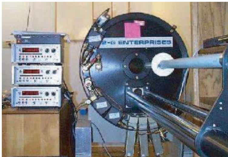
Figure 9.8: a) Cryogenic magnetometer. The sample is inserted into the opening of the shields. There are three SQUIDS that detect the magnetic moment which is read off the three electronic boxes to the left. b) Spinner magnetometer. The sample is inserted into the opening in a cup. It spins around, generating an electromagnetic force which is detected with a circular fluxgate. Two components are measured at a time.
