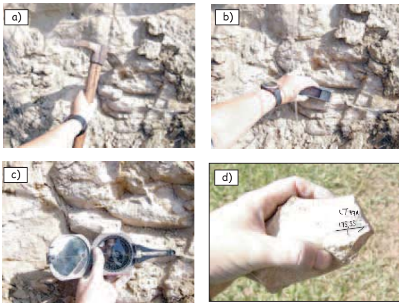
Figure 9.2: Hand sampling technique for soft sediment: a) dig down to fresh material, b) rasp off a flat surface, c) mark the strike and dip on the sample, d) extract the sample and label it.
