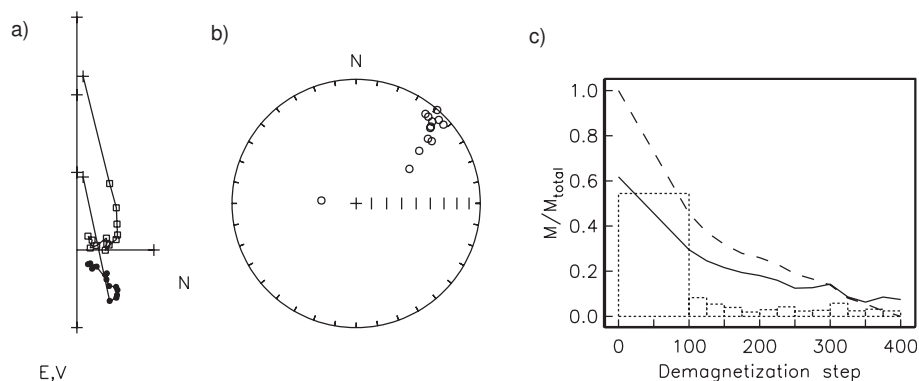
Figure 9.12: a) Specimen with strongly overlapping remanence components, in an orthogonal projection. b) Same data as in a) plotted on an equal area projection. c) Decay of NRM intensity during the demagnetization procedure (solid line). The dashed line is the decay of the vector difference sum. Boxes represent the intensity removed after each step.
