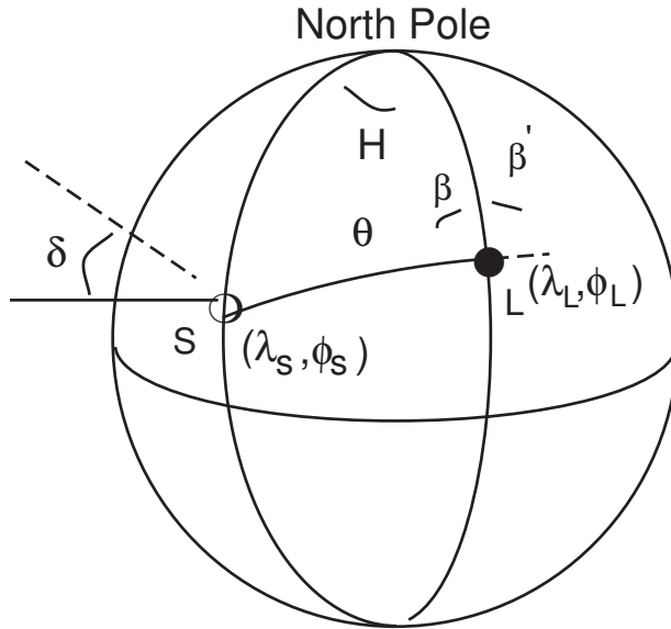
Figure A1: Calculation of the azimuth of the shadow direction ( \beta' ) relative to true North, using a sun compass. L is the site location (at \lambda_L, \phi_L ), S is the position on the Earth where the sun is directly overhead ( \lambda_S, \phi_S ).
