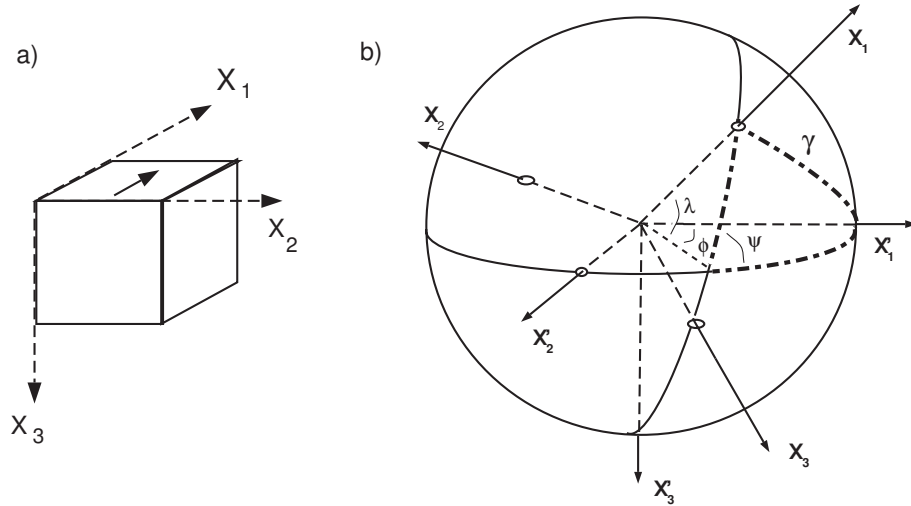
Figure B1: a) Sample coordinate system. b) Trigonometric relations between two cartesian coordinate systems, \mathbf{X}_i and \mathbf{X}'_i . \lambda, \phi, \psi are all known and the angles between the various axes can be calculated using spherical trigonometry. For example, the angle \gamma between \mathbf{X}_1 and \mathbf{X}'_1 forms one side of the triangle shown by dash-dot lines. Thus, \cos \gamma = \cos \lambda \cos \phi + \sin \lambda \sin \phi \cos \psi .
