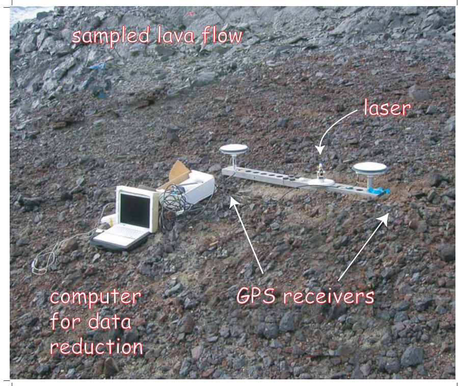
Figure 9.6: Differential GPS system for orienting paleomagnetic samples in polar regions. Photo taken during sampling trip to the foothills of the Royal Society Ranges in Antarctica, Jan. 2004.
