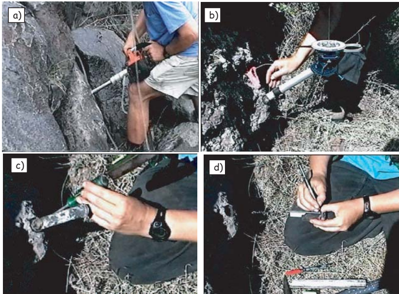
Figure 9.1: Sampling technique with a water-cooled drill: a) drill the sample, b) insert a non-magnetic slotted tube with an adjustable platform around the sample. Rotate the slot to the top of the sample and note the azimuth and plunge of the drill direction (into the outcrop) with a sun and/or magnetic compass and inclinometer. Mark the sample through the slot with a brass or copper wire. c) Extract the sample. d) Make a permanent arrow on the side of the sample in the direction of drill and label the sample with the sample name. Make a note of the name and orientation of the arrow in a field notebook.
