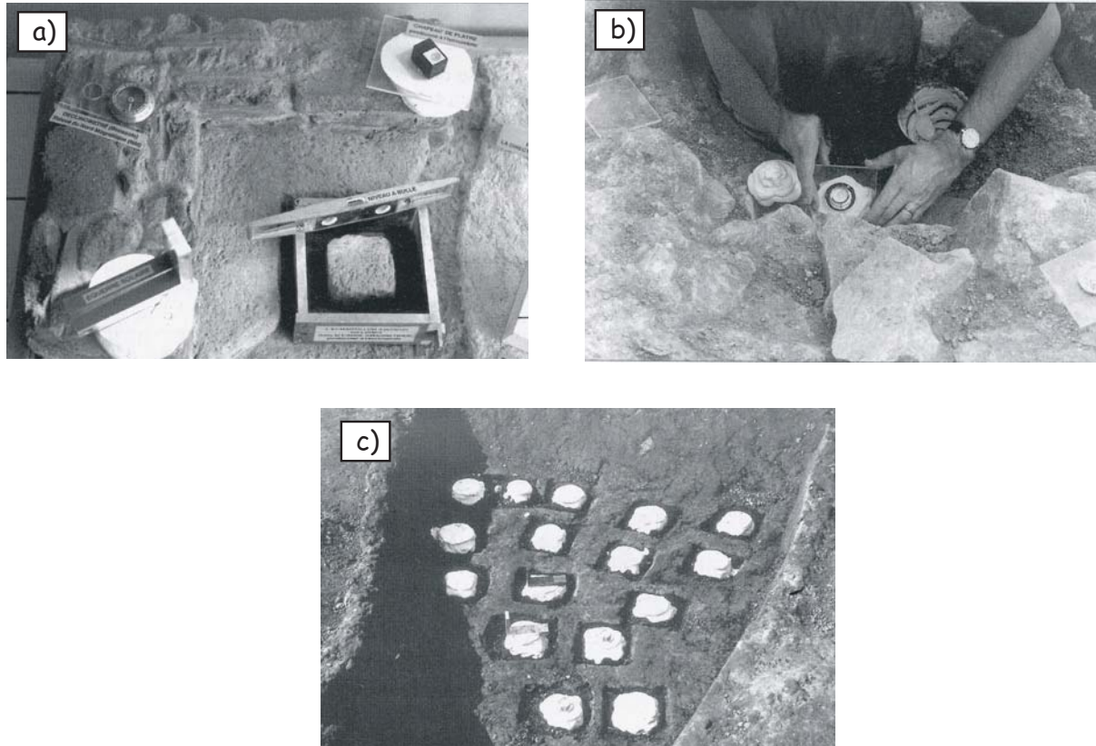
Figure 9.3: Sampling technique for oriented archeological materials. a) cut out a large sample from, for example, a baked hearth. b) cover the sample with non-magnetic plaster of paris. While the plaster of paris is still wet, place a piece of plexiglass on it and orient it such that it is horizontal using a bubble level. c) The direction to magnetic north can be inscribed on the horizontal surface, after the plaster is dry. [Picture from Evin et al. 1998]
