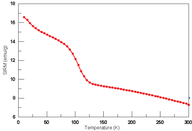
Figure 4.3: Magnetization curve for magnetite as a function of temperature. As the sample goes through the Verwey transition, a fraction of the magnetization is lost. Figure modified from the “Rock magnetic Bestiary” collection at the Institute for Rock Magnetism.
