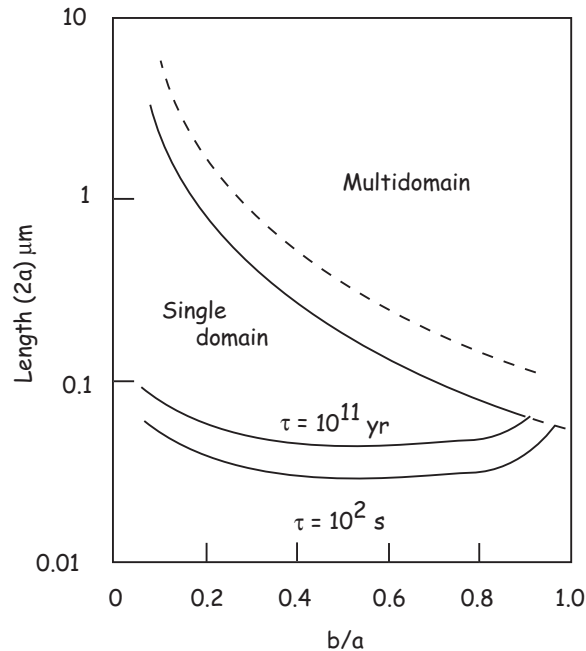
Figure 4.13: Expected domain states for various sizes and shapes of parallelepipeds of magnetite at room temperature. a and b are as in Figure 4.4. [Figure redrawn from Evans and McElhinny, 1969.]
