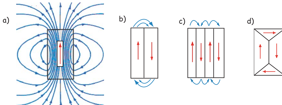
Figure 4.8: A variety of domain structures of a given particle. a) Uniformly magnetized (single domain). b) Two domains. c) Four domains in a lamellar pattern. d) Essentially two domains with two closure domains.
