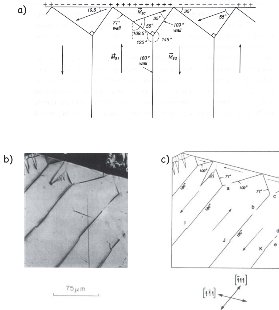
Figure 4.11: a) Theoretical predictions of possible domain structures for magnetite. b) Bitter patterns from an oriented polished section of magnetite. c) Interpretation of the magnetization. [Figures from Dunlop and Ozdemir (1997)].
