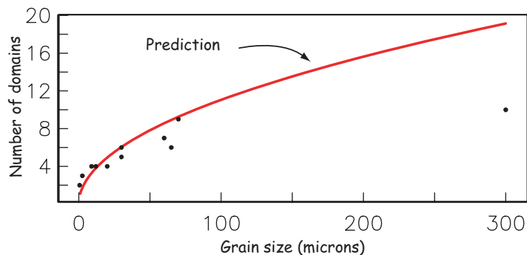
Figure 4.12: Number of domains in magnetite particles versus grain size. Solid curve: predicted values from theory (see text). Dots: data compiled by Özdemir and Dunlop (1997).
