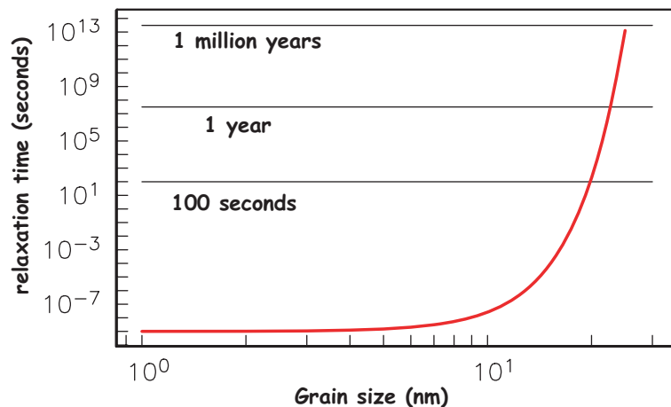
Figure 4.5: Relaxation time as a function of grain size in nanometers.
