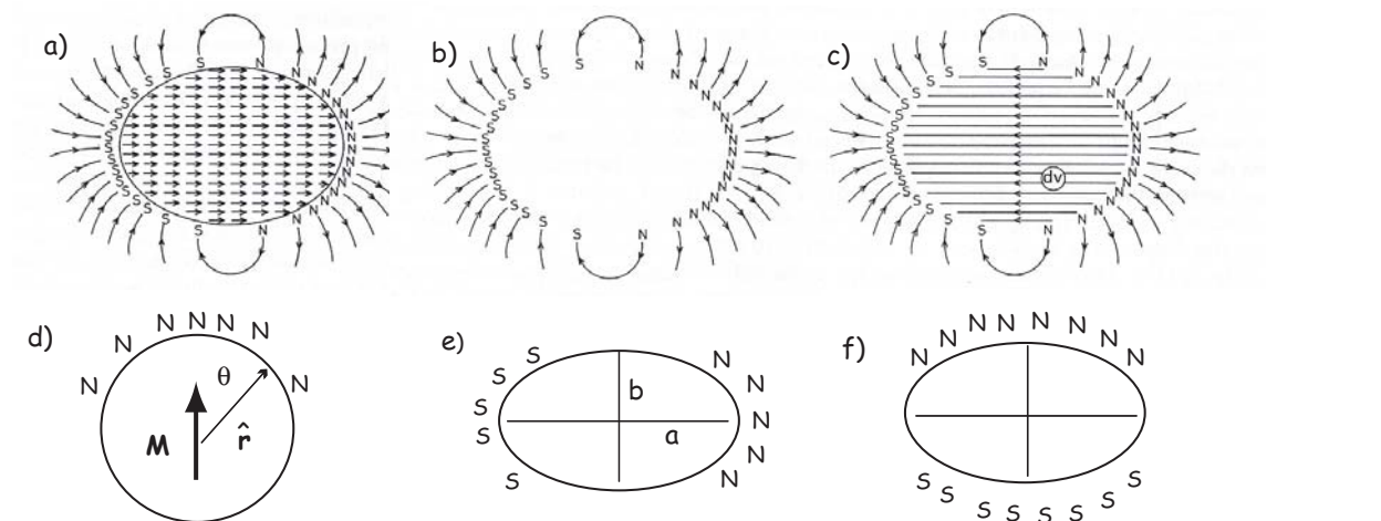
Figure 4.4: a) Internal magnetizations within a ferromagnetic crystal. b) Generation of an identical external field from a series of surface monopoles. c) The internal “demagnetizing” field resulting from the surface poles. (Redrawn from O’Reilly [1984]). d) Surface poles on a sphere. e) Surface poles on an ellipse, with the magnetization parallel to the elongation. f) Surface poles with the magnetization perpendicular to the axis of elongation.
