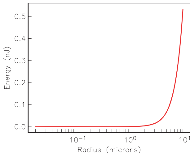
Figure 4.6: The self energy of a spherical particle of magnetite as a function of particle radius.
