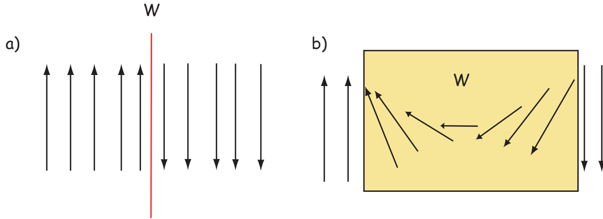
Figure 4.9: Examples of possible domain walls. a) There is a 180^\circ switch from one atom to the next. The domain wall is very thin, but the exchange price is very high. b) There is a more gradual switch from one direction to the other [note: each arrow represents several 10 's of unit cells]. The exchange energy price is lower, but there are more spins in unfavorable directions from a magnetocrystalline point of view.
