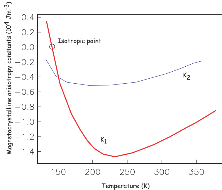
Figure 4.2: Variation of K_1 and K_2 of magnetite as a function of temperature. Redrawn from Dunlop and Özdemir (1997).
