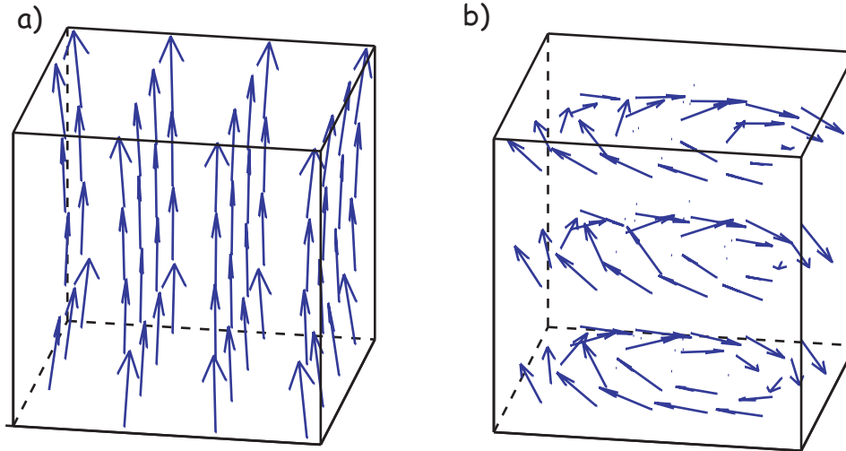
Figure 4.7: Possible non-uniform magnetization configurations that reduce self energy for magnetite with increasing particle widths. a) “Flower” state, b) “Vortex” state. (From Tauxe et al., 2002)
