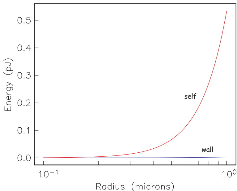
Figure 4.10: Comparison of “self” energy versus the energy of the domain wall in magnetite spheres as a function of particle size.
