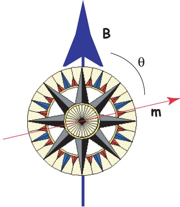
Figure 1.4: A magnetic moment \mathbf{m} of for example a compass needle, will tend to align itself with a magnetic field \mathbf{B} . The aligning energy is the magnetostatic energy which is greatest when the angle between the two vectors \theta is at a maximum.
