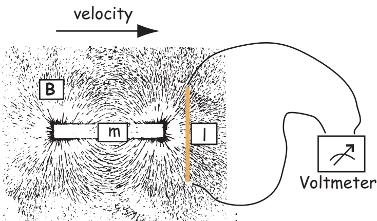
Figure 1.3: A magnetic moment \mathbf{m} makes a vector field \mathbf{B} made visible by the iron filings. If this field moves with velocity \mathbf{v} , it generates a voltage V in an electrical conductor of length l . [Iron filings picture from Jiles (1992).]
