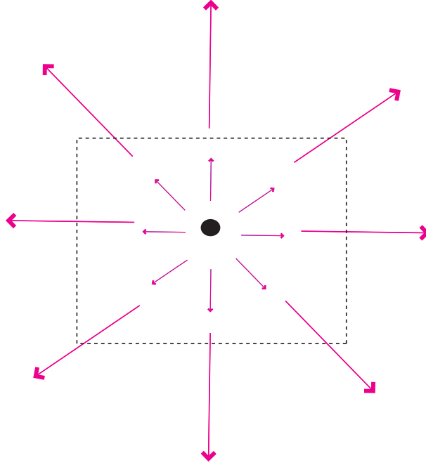
Figure B2: Example of a vector field with a non-zero divergence.
