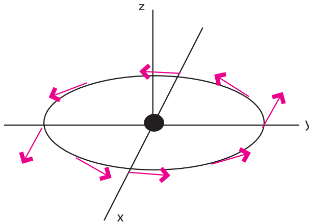
Figure B4: Example of a vector field with non-zero curl.
