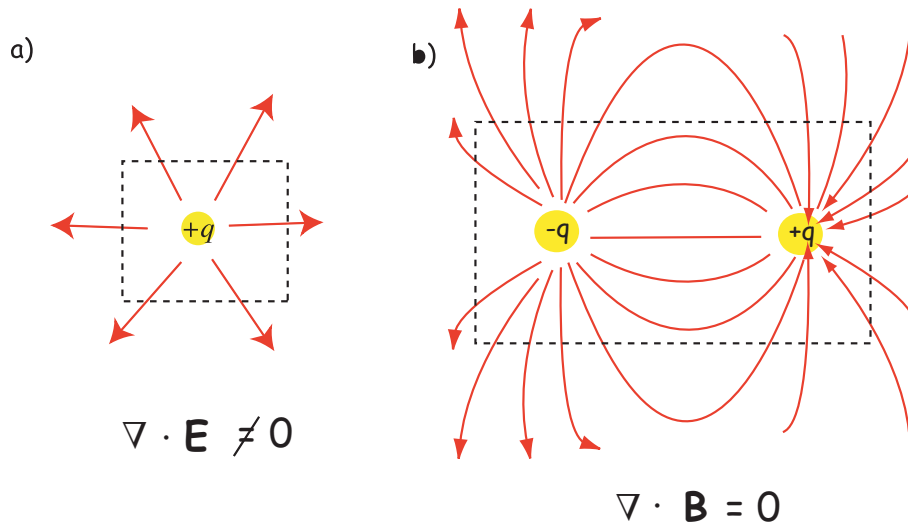
Figure 1.5: a) An electric charge produces a field that diverges out from the source. There is a net flux out of the dashed box, quantified by the divergence ( \nabla \cdot \mathbf{E} ), which is proportional to the magnitude of the sources inside the box. b) there are no isolated magnetic charges, only dipoles. Within any space (e.g., the dashed box) any flux line that comes in, goes out. The divergence of such a field is zero, i.e., \nabla \cdot \mathbf{B} = 0 .
