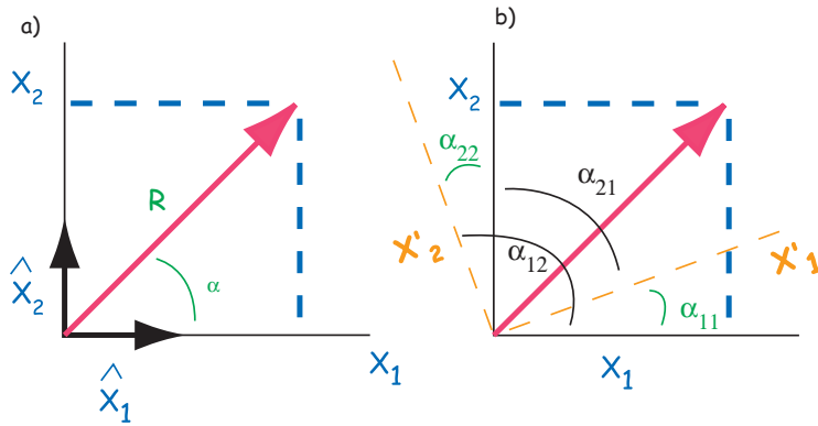
Figure A3: Transformation of axes. a) Definition of vector in one set of coordinates, x_1, x_2 . b) Definition of angles relating old X axes to new X' .
