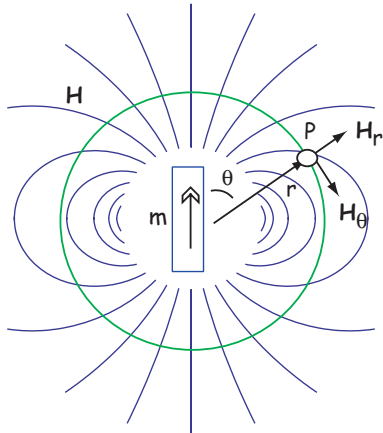
Figure 1.6: Field \mathbf{H} produced at point P by a magnetic moment \mathbf{m} . \mathbf{H}_r and \mathbf{H}_\theta are the radial and tangential fields respectively.
