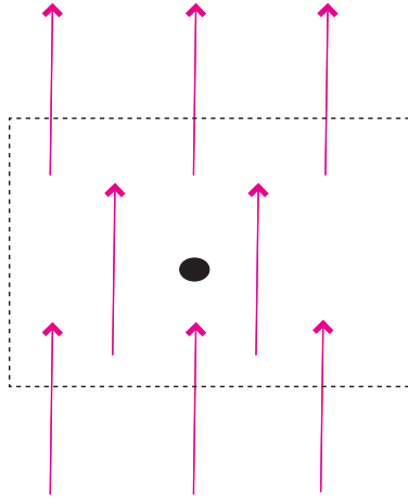
Figure B3: Example of a vector field with zero divergence.
