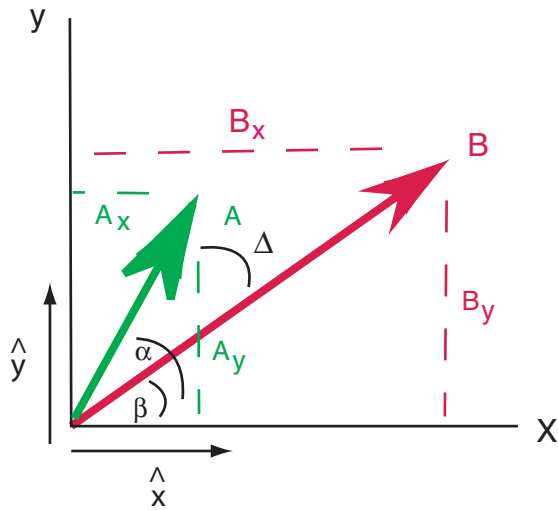
Figure A1: Vectors \mathbf{A} and \mathbf{B} , their components A_{x,y} , B_{x,y} and the angles between them and the X axis, \alpha and \beta . The angle between the two vectors is \alpha - \beta = \Delta . Unit vectors in the directions of the axes are \hat{x} and \hat{y} respectively.
