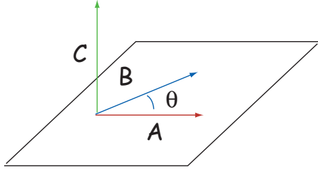
Figure A2: Illustration of cross product of vectors A and B separated by angle \theta to get the orthogonal vector C .
