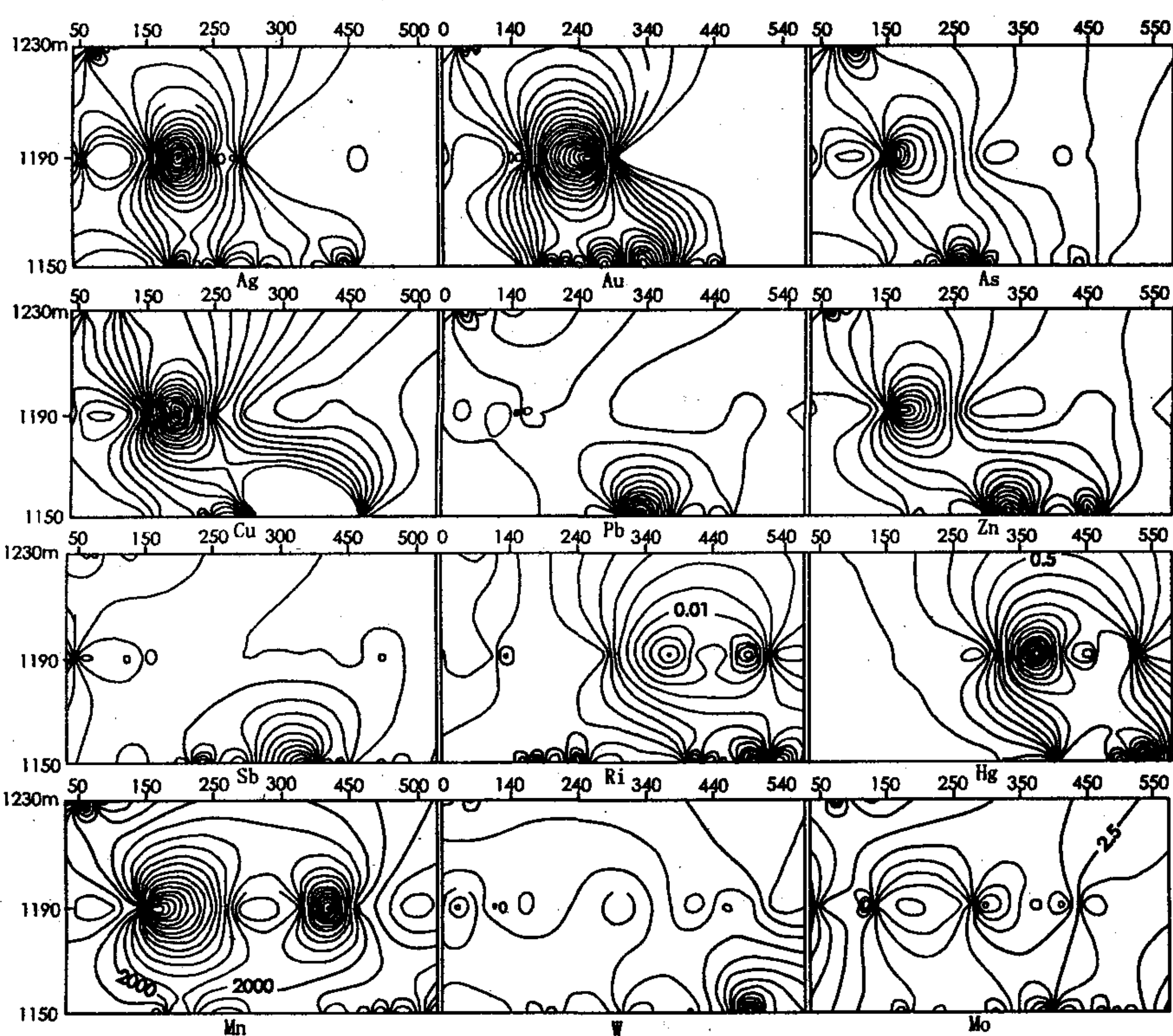
图 1 丰宁银矿指示元素品位剖面等值线图 Fig. 1 The grade isoline profile of indication elements, Fengning silver deposit
