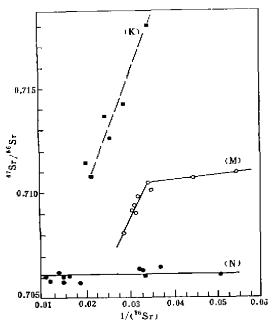
图5 牛头山玄武岩的 ^{87}\text{Sr}/^{86}\text{Sr} - 1/(^{86}\text{Sr}) 图 N为牛头山玄武岩, M为月球火山口熔岩和 K为国王山玄武岩 (据Briqueu和Lancelot, 1979) Fig.5 Relationship between ^{87}\text{Sr}/^{86}\text{Sr} and 1/^{86}\text{Sr} for Niutoushan basalts (for King hill basalts and crater of the Moon lavas, after Briqueu and Lancelot, 1979)
