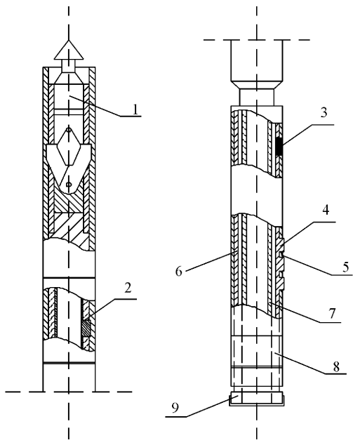
图 1 DQ-76 型连续造斜绳索取心钻具结构示意图 Fig.1 Schematic diagram showing structure of DQ76 continuous deflecting wire-line coring tool assembly 1-打捞机构;2-仪器管;3-分动机构;4-卡固块;5-卡固管;6-传扭管;7-取心内管;8-造斜机构;9-取心钻头 1- salved set; 2- measurement house; 3- action set; 4- locking block; 5- locking house; 6- drive tube; 7- core barrel; 8- deflecting set; 9- coring bit
