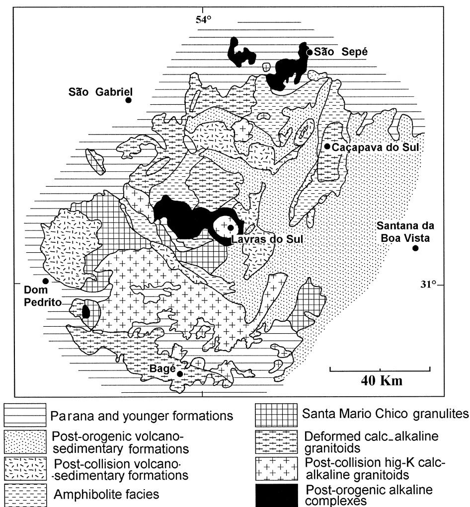
Fig. 3. The Sul-rio-grandense shield (Bitencourt et al., 1987; Nardi and Bonin, 1991).
