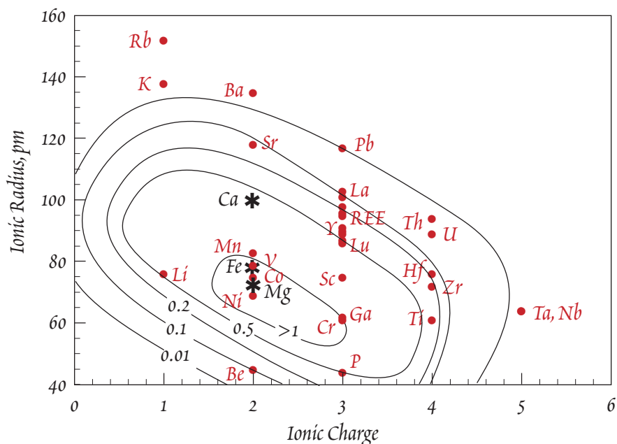
Figure 7.10. Ionic radius (picometers) vs. ionic charge contoured for clinopyroxene/liquid partition coefficients. Cations normally present in clinopyroxene are \text{Ca}^{2+} , \text{Mg}^{2+} , and \text{Fe}^{2+} , shown by * symbols. Elements whose charge and ionic radius most closely match that of the major elements have the highest partition coefficients.
