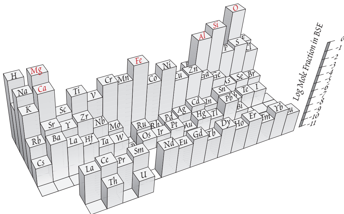
Figure 7.1. Three dimensional histogram illustrating the abundance of the elements (as the log of mole fraction) in the silicate portion of the Earth (the “Bulk Silicate Earth”; BSE). Just 6 elements, oxygen, magnesium, silicon, iron, aluminum, and calcium make up 99.1% of the silicate Earth. If we include the core and consider the composition of the entire Earth, then only nickel, and perhaps sulfur, need be added to this list. The remaining elements, though sometimes locally concentrated (e.g., in the crust, in the hydrosphere, in ores) can be considered trace elements .
