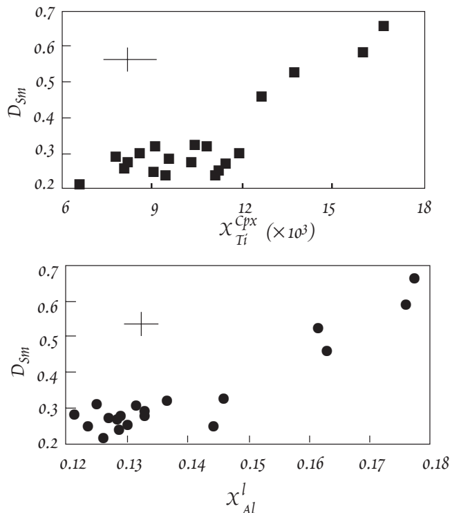
Figure 7.14. Experimentally determined clinopyroxene–liquid partition coefficient for Sm as a function of the mole fraction of Al in the melt and the mole fraction of Ti in cpx. The correlation with Ti suggests Ti and REE partitioning is controlled by similar factors. Cross shows analytical error. From Gallahan and Nielsen (1992).
