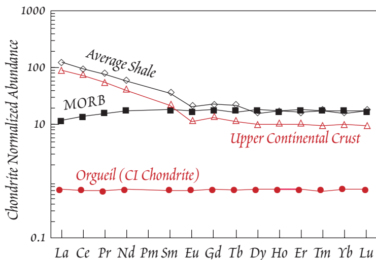
Figure 7.7. A rare earth plot showing rare earth patterns for average upper continental crust (Rudnick and Fountain, 1995) and average mid-ocean ridge basalt.
