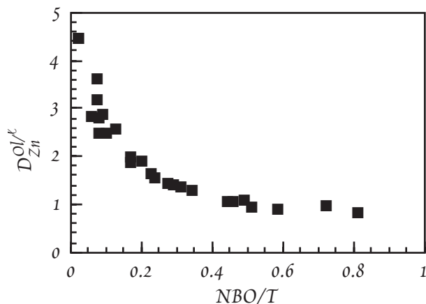
Figure 7.12. Variation of the zinc olivine/liquid partition coefficient as a function of the number of non-bridging oxygens per tetrahedral cation (NBO/T) in experiments by Kohn and Schofield (1994).
