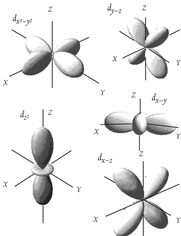
Figure 7.16. Geometry of the d orbitals. In an isolated first series transition metal, the 5 3d orbitals (each containing up to 2 electrons: a total of 10 electrons are possible in the d orbitals) are energetically equivalent and have equal probability of being filled: they are said to be degenerate . They possess, however, different spatial configurations (Figure 7.16). One group, the e_g orbitals, consisting of the d_{z^2} and the d_{x^2-y^2} orbitals, has lobes directed along the Cartesian coordinates, while the t_{2g} group, consisting of the d_{xy} , d_{yz} , and d_{xz} , possess lobes between the Cartesian axes. In a crystal field the 3d orbitals are no longer degenerate, and some have lower energy than others. Thus there can be a relative energy gain by preferentially filling low-energy d orbitals. This energy gain is traded off against the energy cost of placing two electrons in a single orbital. Depending on this trade off, preferentially filling low energy d orbitals can lower the overall energy of some transition metal ions, hence stabilizing them, in certain lattice configurations relative to other configurations. The effect is a lattice site preference of some transition metals that would not be predicted simply from consideration of ion charge and size.
