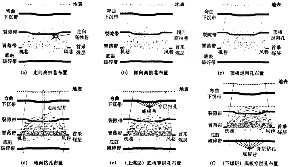
图 10 被保护层卸压瓦斯抽采图例 Fig. 10 Pressure-relief gas drainage in protected coal seams
