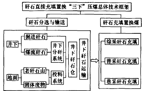
图 18 矸石充填置换煤总体技术框图 Fig. 18 General technological framework of coal replacement with waste rock
