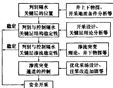
图 13 保水采煤的隔水关键层原理 Fig. 13 Principle of WKS in water-preserved mining
