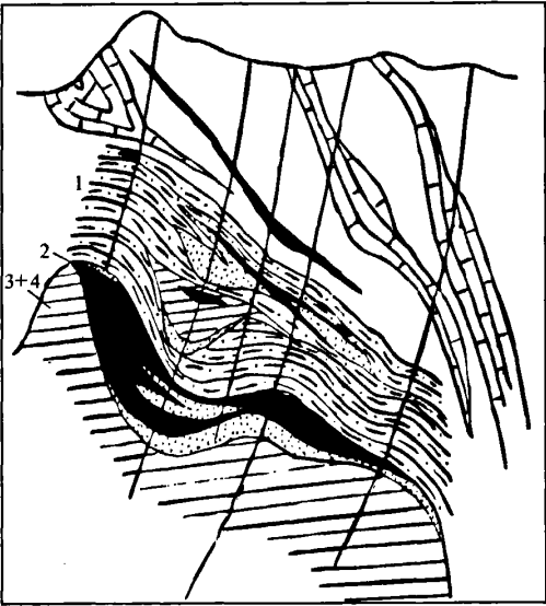
图 7 毕家山铅锌矿礁硅岩套典型剖面(据李建中,1983) Fig. 7 Representative section showing the combination of reef and quartzite (after Li, 1983)
