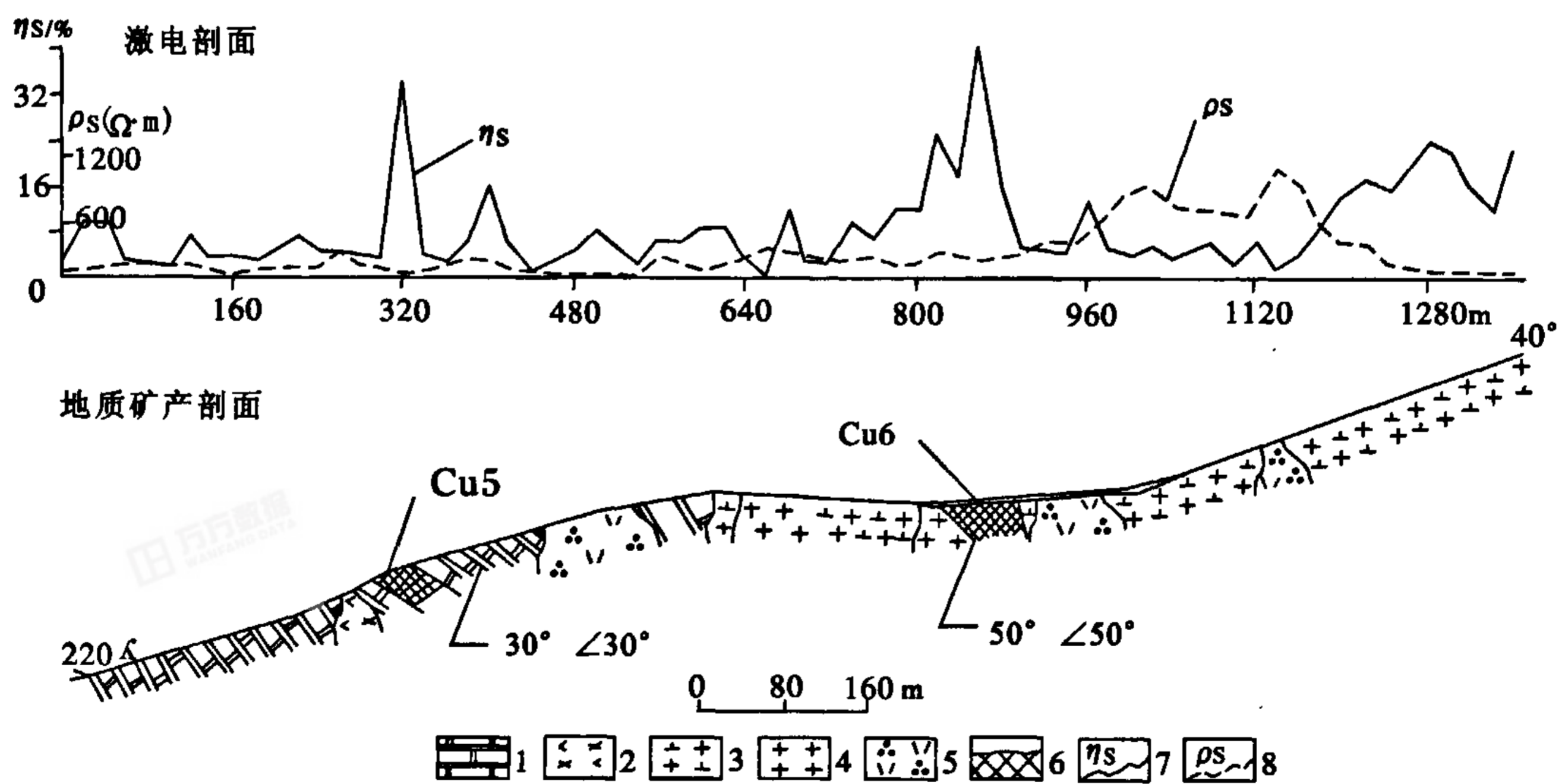
图 2 措勤县日阿 60 线综合地质剖面图 1—大理岩;2—角闪辉长岩;3—花岗闪长岩;4—花岗斑岩;5—石英斑岩; 6—铜矿化体;7—视极化率曲线;8—视电阻率曲线 Fig.2 Composite geological section along line 60 of Ri'a, Coqên County 1-Marble;2-Hornblende gabbro;3-Granodiorite;4-Granite porphyry; 5-Quartz porphyry;6-Copper mineralization body; 7-Apparent polarizability curve; 8-Apparent resistivity curve
