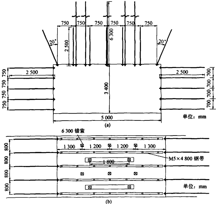
图 3 巷道锚杆(索)支护布置图 Fig.3 Distribution sketch of bolting(cable) for roadway
