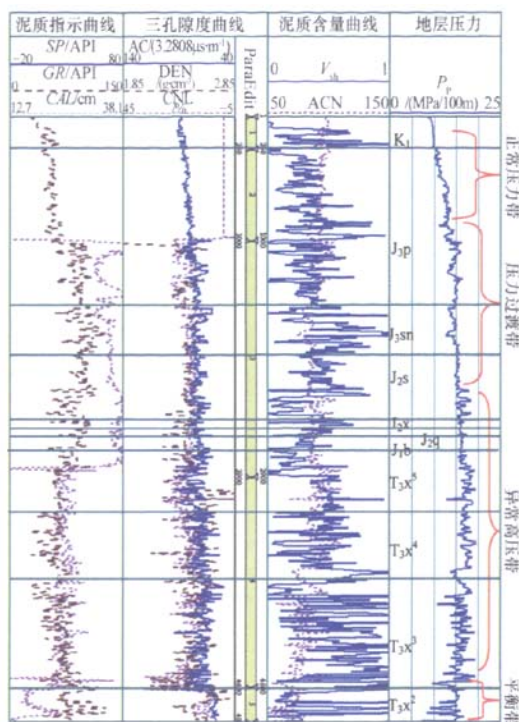
图7 X851井地层孔隙压力剖面 Fig. 7 Pore pressure profile of X851
