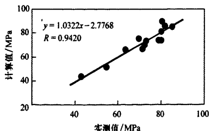
图6 地层孔隙压力实测值与计算值对比 Fig. 6 Measured and calculated pore pressures
