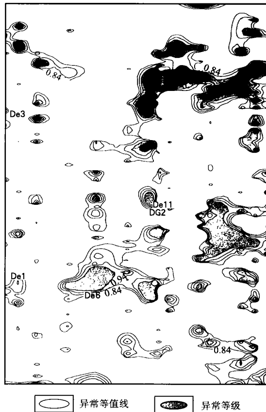
图 6 工区沙三 2 层油气异常分布图 Fig. 6 Distribution of geo-anomalies of oil and gas of the Es 3-2 layer in study area
