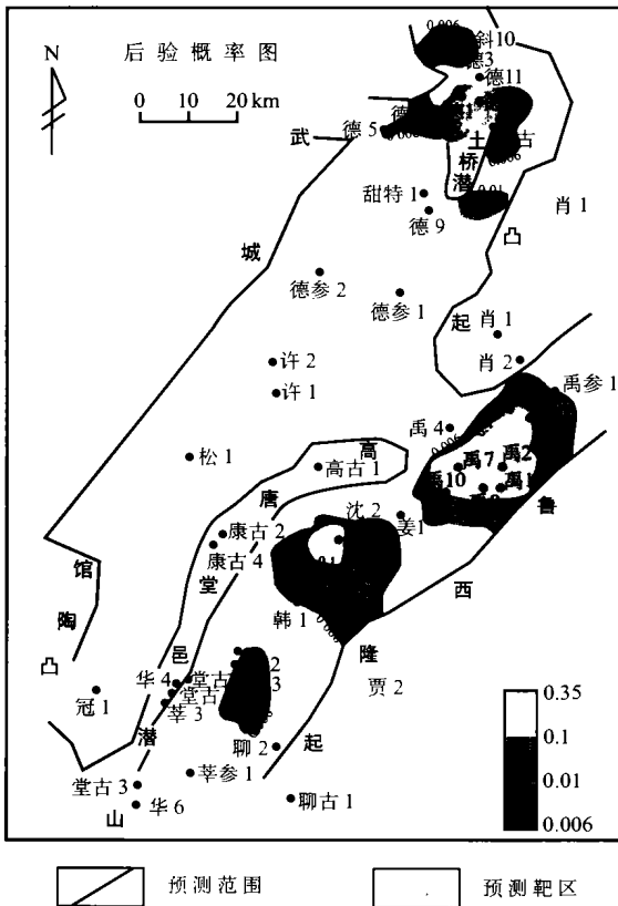
图 5 区 m 域油气地质异常有利地带预测图 Fig. 5 Prognostic chart of the preferable areas of geo-anomalies of oil and gas
