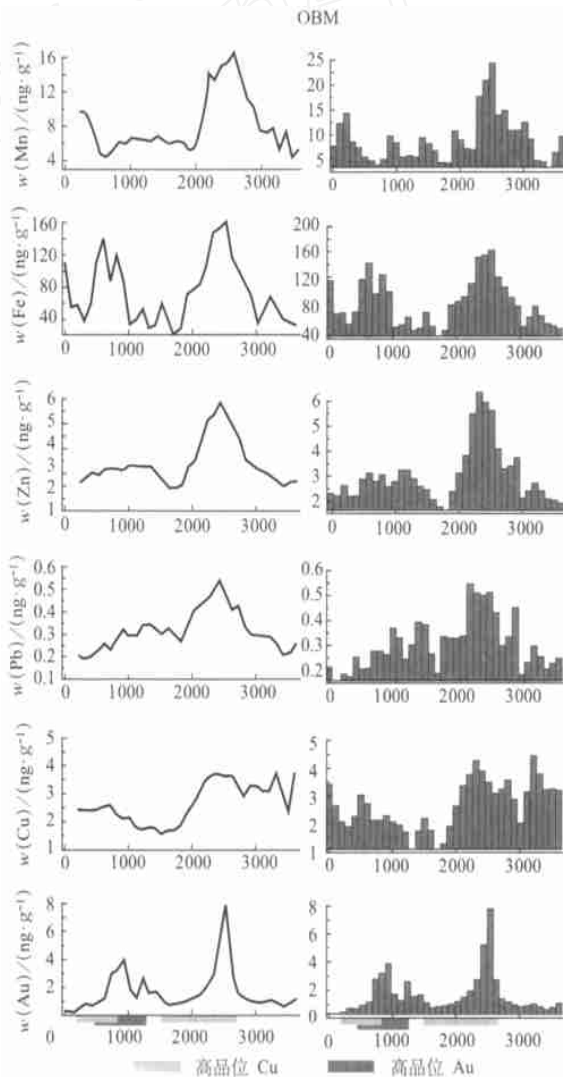
图 9 用距离倒数移动平均法处理数据后 Au, Cu, Zn, Pb, Fe, Mn 在 Mike 矿床上的异常 Fig. 9 OBM anomalies of Au, Cu, Pb, Zn, Fe and Mn over Mike deposit (plotted after data treatment by inverse distance moving average method)
